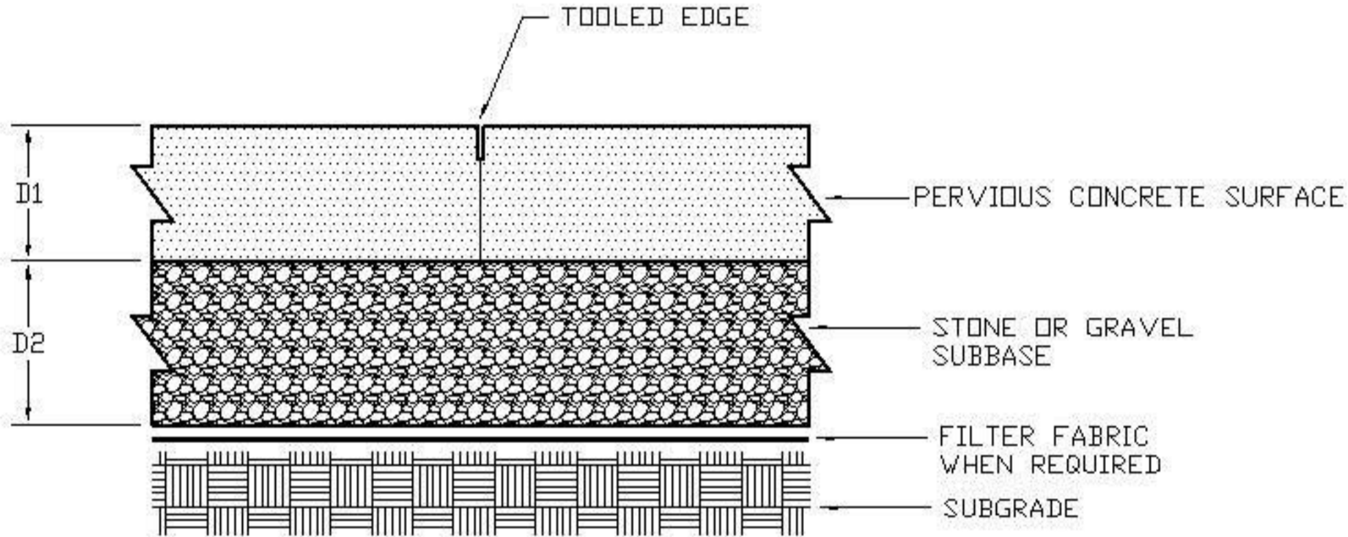
PERVIOUS CONSTRUCTION JOINT
