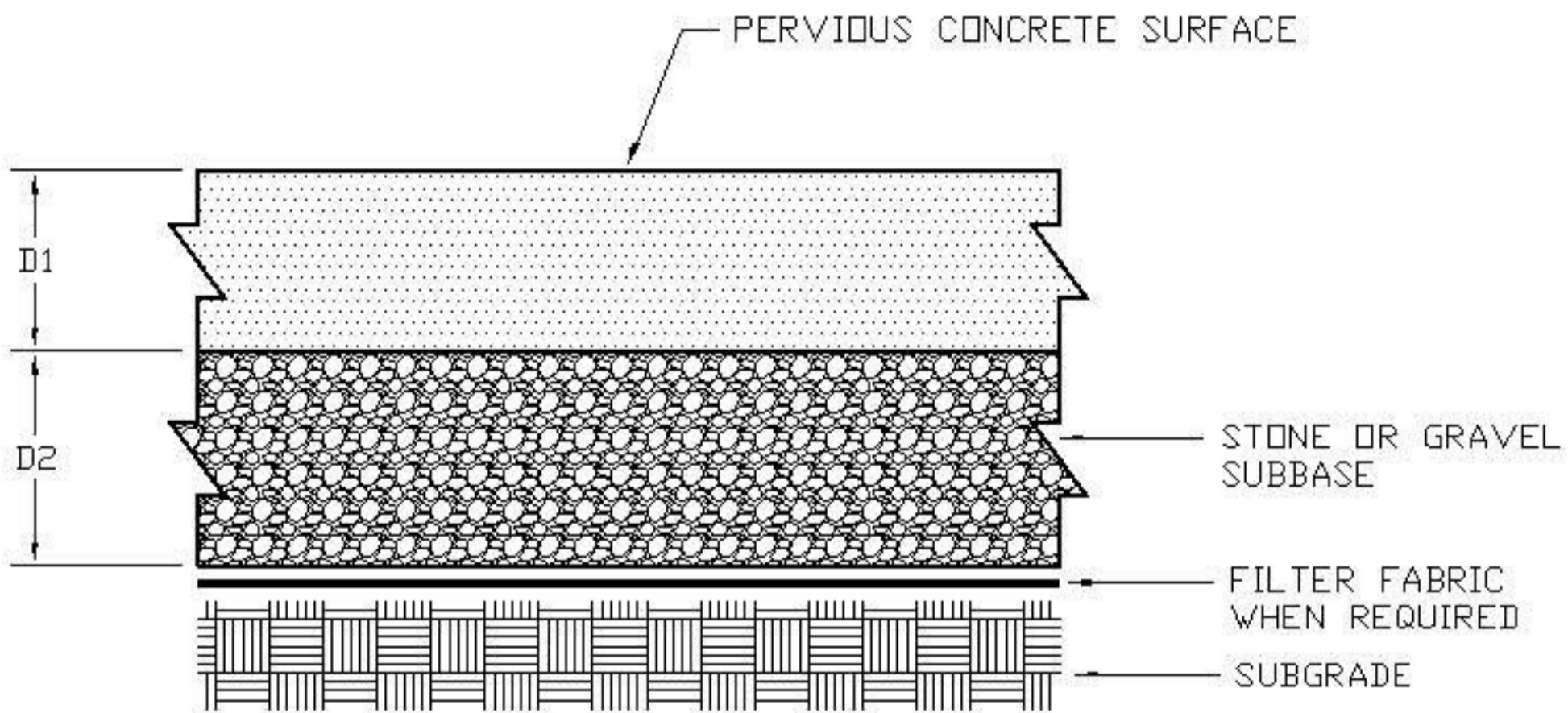
PERVIOUS TYPICAL SECTION
